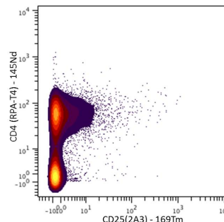
Human PBMCs stained with 145Nd-anti-CD4 (RPA-T4) and 169Tm-anti-CD25 (2A3). CD3+ CD20- cells are displayed in the analysis.
