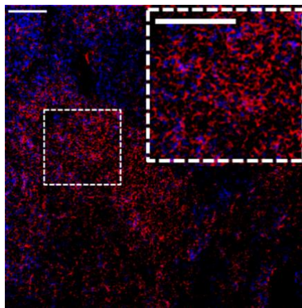
Human frozen tonsil stained with 158Gd-anti-CD45RA (HI100) at a dilution of 1:100 (red pseudocolor) and iridium DNA intercalator (blue pseudocolor). Tissue section was fixed in 4% paraformaldehyde for 30 minutes at 4 °C. Scale bar size = 100 µm.
