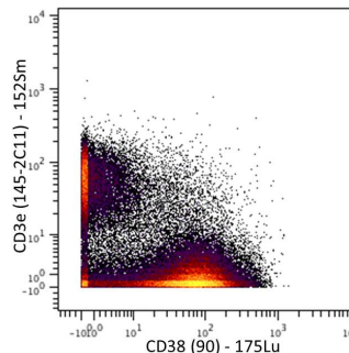
C57BL/6 mouse splenocytes stained with 152Sm-anti-CD3e (145-2C11) and 175Lu-anti-CD38 (90).
